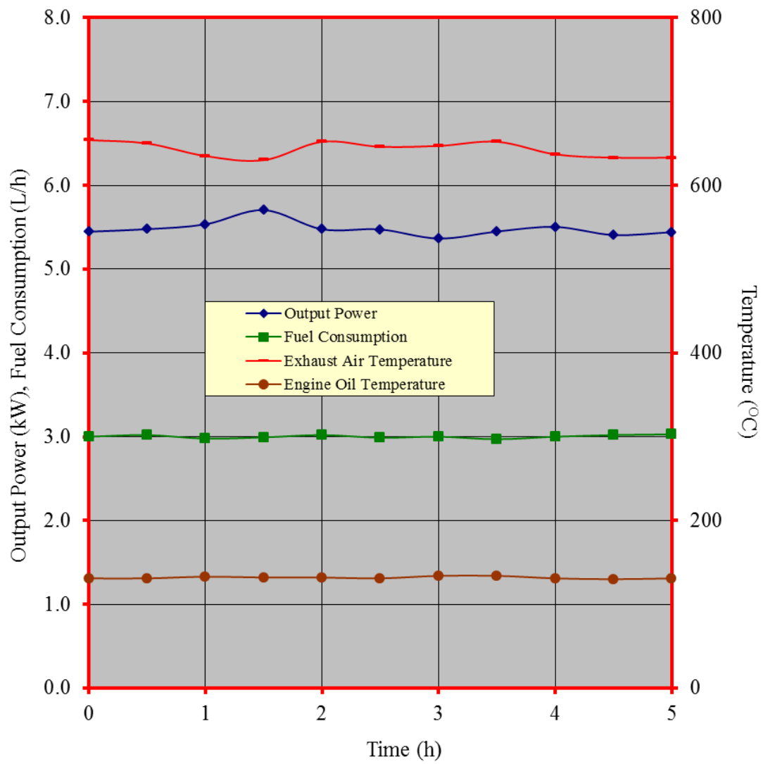
Figure 4. Performance characteristic curves during the continuous running test of the MITSUBISHI GB300PN-RSM Gasoline engine
