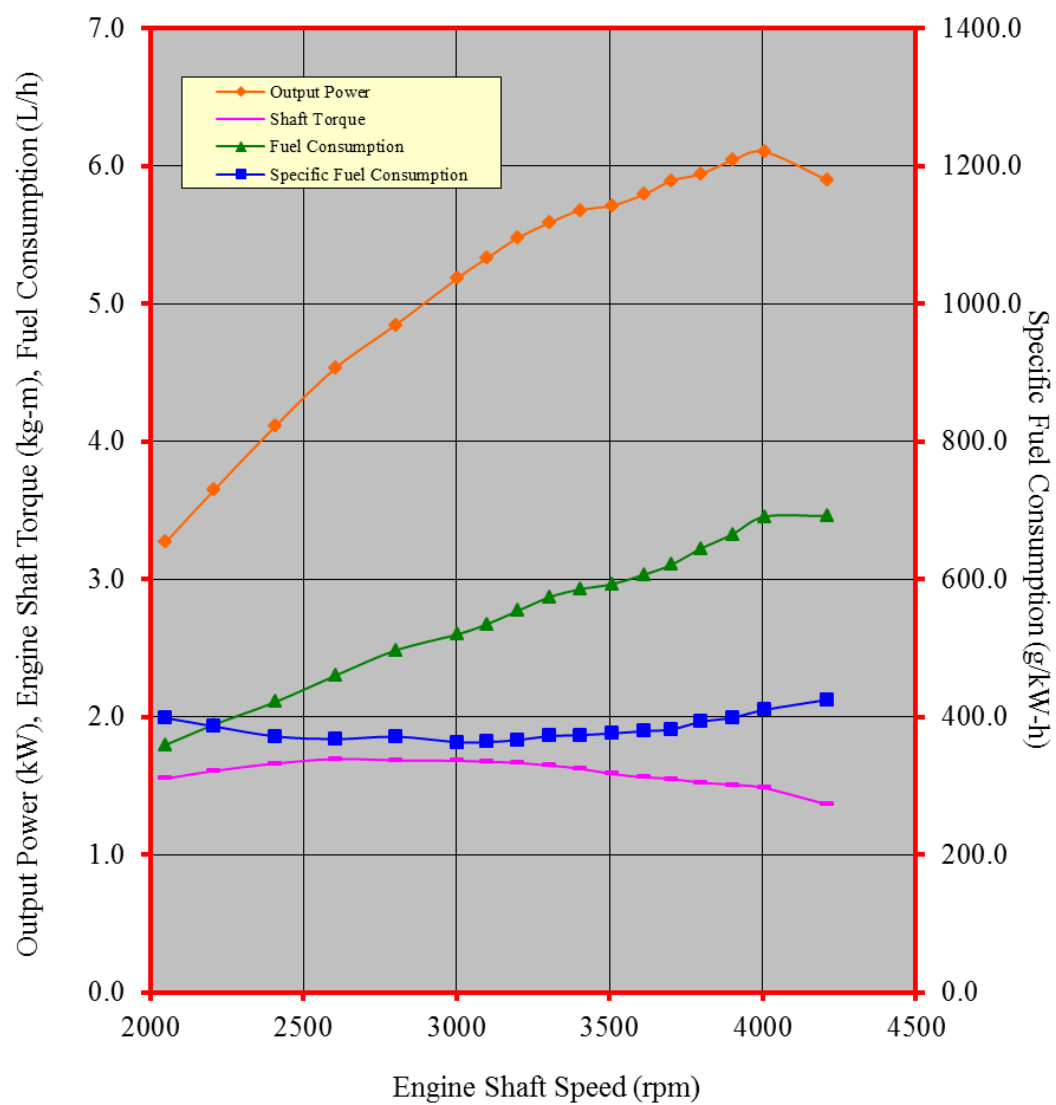
Figure 3. Performance characteristic curves of the MITSUBISHI GB300PN-RSM gasoline engine (B)
